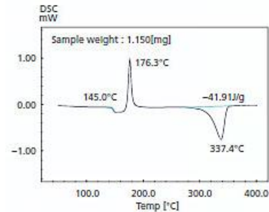
Measurement of Engineering Plastic (PEEK)
